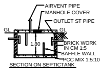
SECTION ON SEPTICTANK
