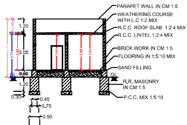
SECTION OF "AB"
