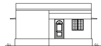
FRONT ELEVATION
