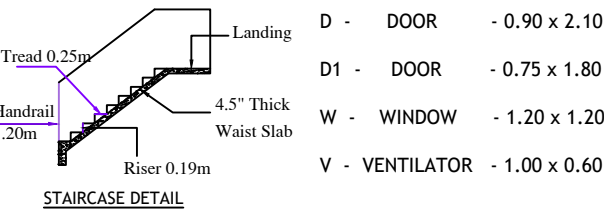
STAIRCASE DETAIL
