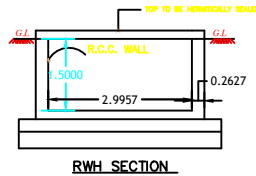
RWH SECTION
