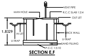
SEPTIC TANK DETAIL
