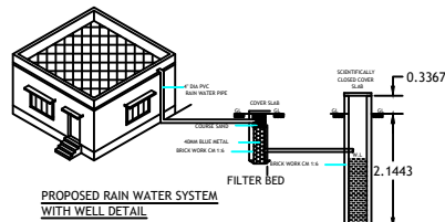
PROPOSED RAIN WATER SYSTEM WITH WELL DETAIL
