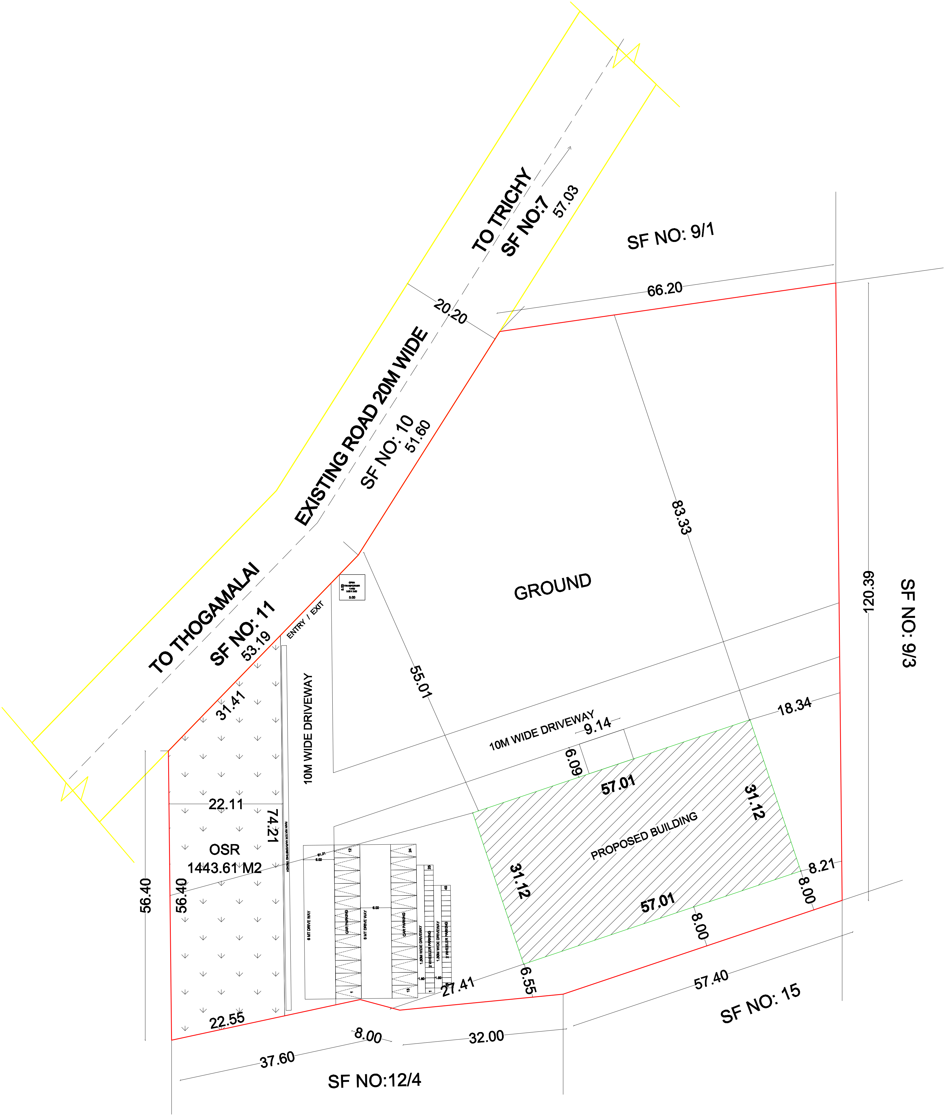
SITE PLAN
