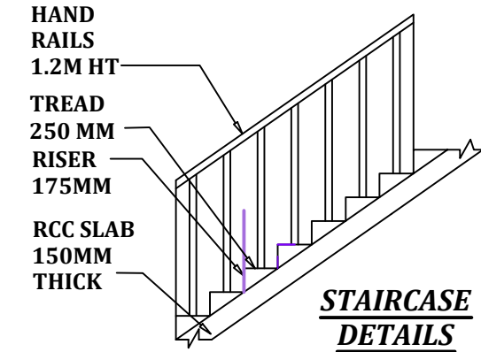
STAIRCASE DETAILS SCALE 1:50
