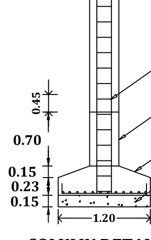
COLUMN DETAILS SCALE 1:50
