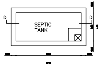
PLAN OF SEPTIC TANK SCALE 1"=2'0"
