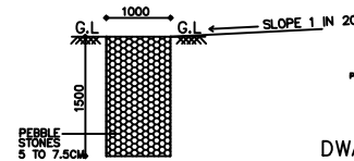
SECTION OF PEBBLE TRENCH SCALE : 1" = 100
