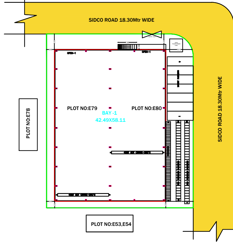
SITE PLAN
