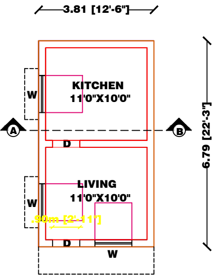
PLAN
