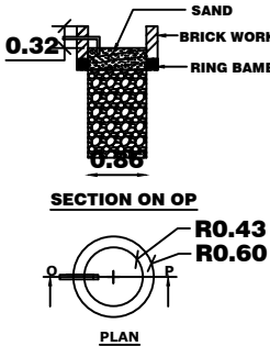
RAIN WATER PIT
