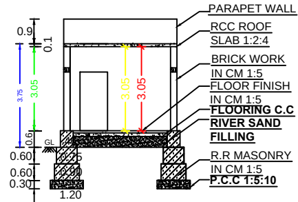
SECTION ON AA1
