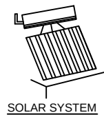
SOLAR SYSTEM
