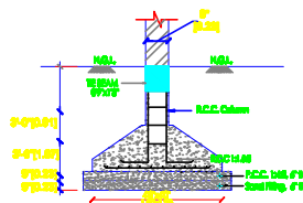
FOUNDATION DETAIL
