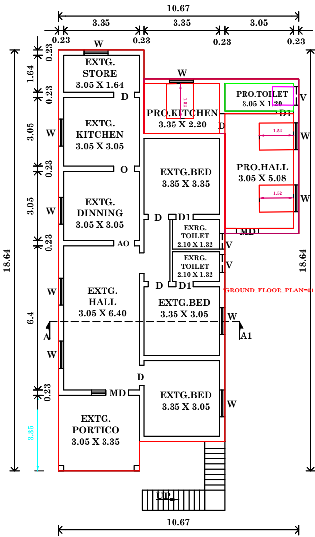
EXISTING AND PROPOSED GROUND FLOOR PLAN
