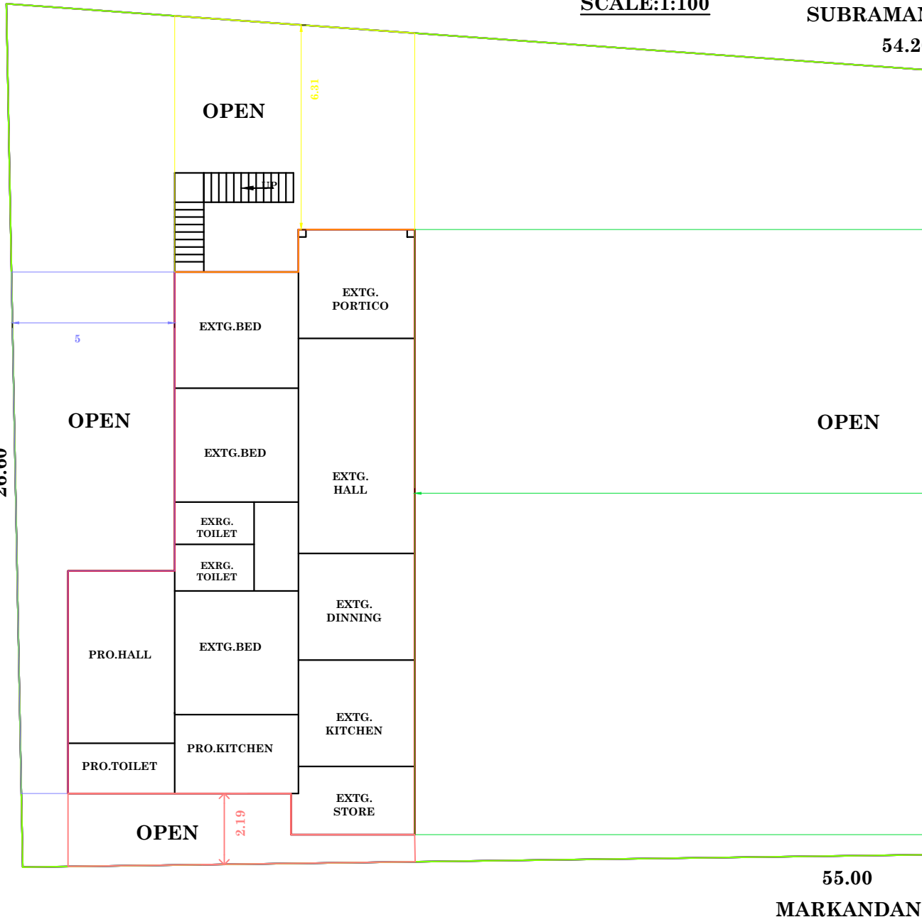
EXISTING AND PROPOSED GROUND FLOOR PLAN
