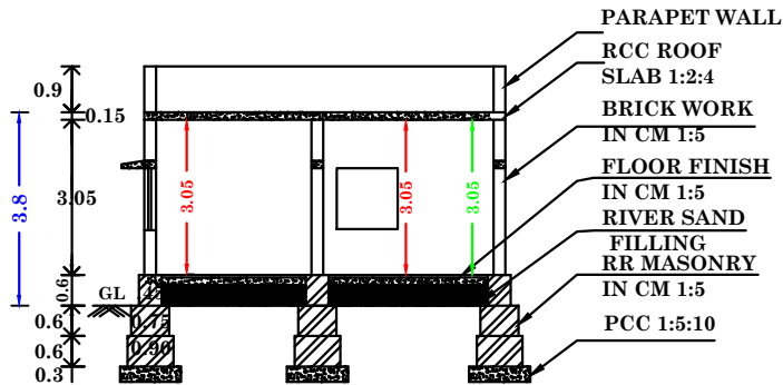
SECTION ON AA1
