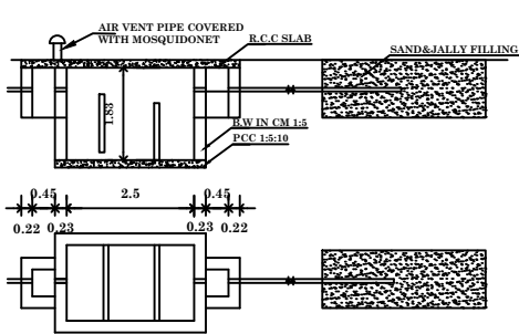
PLAN&SECTION OF SEPTIC TANK TRENCH
