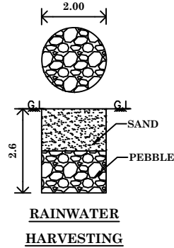
RAINWATER HARVESTING
