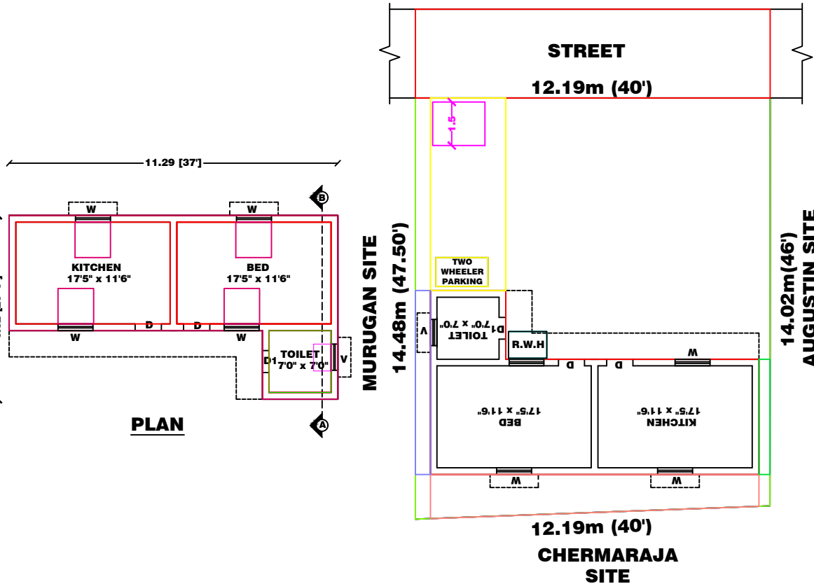
SITE PLAN
