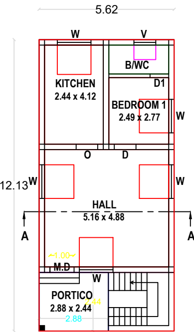
PLAN - GROUND FLOOR
