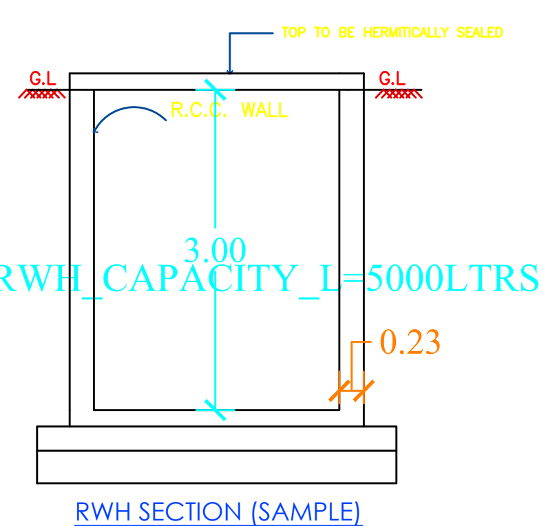
RWH SECTION (SAMPLE)
