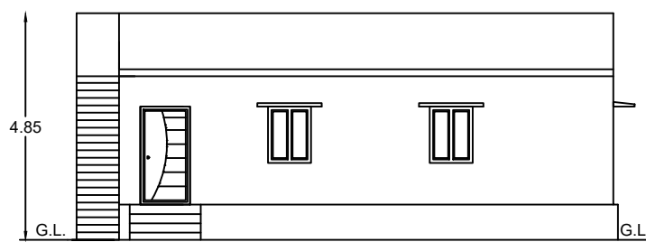
FRONT ELEVATION
