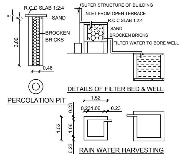
RAIN WATER HARVESTING
