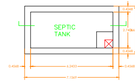
PLAN OF SEPTIC TANK SCALE 1"=2'0"
