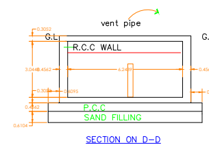
SECTION ON D-D
