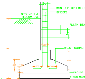
TYPICAL SECTION OF R.C.C COLUMN FOUNDATION SCALE : 1" = 2'-0"
