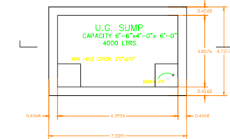
SUMP DETAIL SCALE 1"=4'0"
