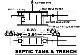
SEPTIC TANK & TRENCH
