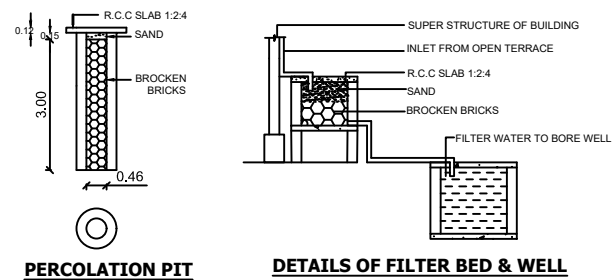
PERCOLATION PIT
