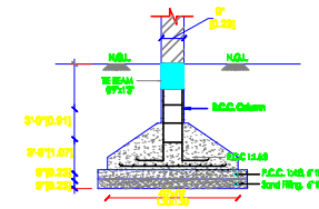
FOUNDATION DETAIL
