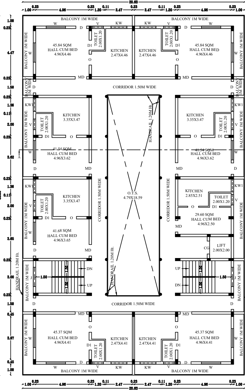
TYPICAL FLOOR PLAN FIRST & SECOND FLOOR PLAN TYPICAL FLOOR PLAN-1,2
