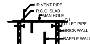
SECTION ON SEP. TANK.
