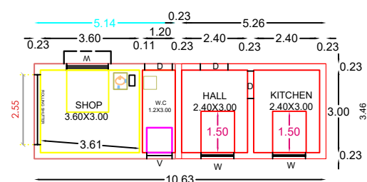
GROUND FLOOR COMMERCIAL CUM RESIDENTIAL PLAN
