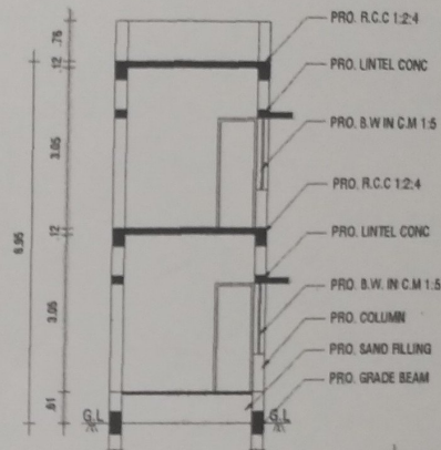
SECTION ON XX
