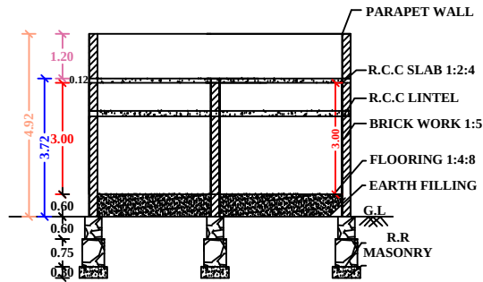
"SECTION AB"
