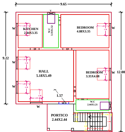
G.F. PLAN
