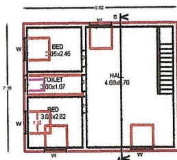
PRO. FIRST FLOOR PLAN
