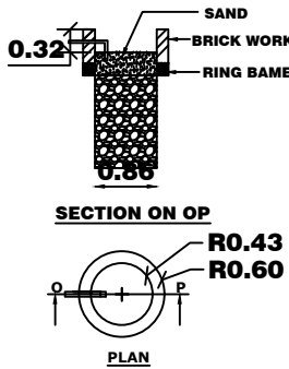
RAIN WATER PIT
