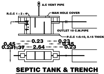
SEPTIC TANK & TRENCH
