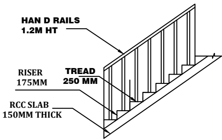
STAIRCASE DETAILS SCALE 1:50
