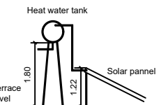
SIDE ELEVATION
