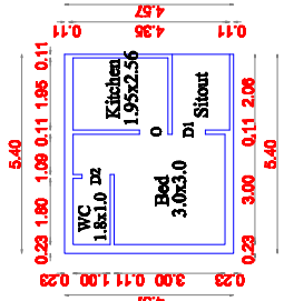
PRO FIRST FLOOR
