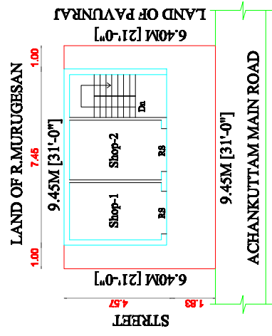
SITE CUM EXISTING GROUND FLOOR
