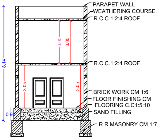
SECTION ON SV
