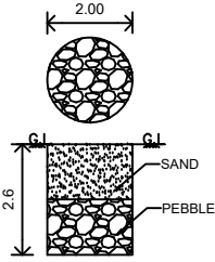
RAINWATER HARVESTING
