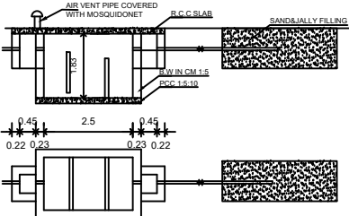
PLAN&SECTION OF SEPTIC TANK TRENCH
