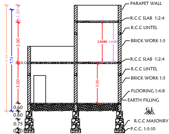
"SECTION "AB"
