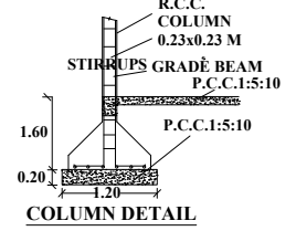
COLUMN DETAIL
