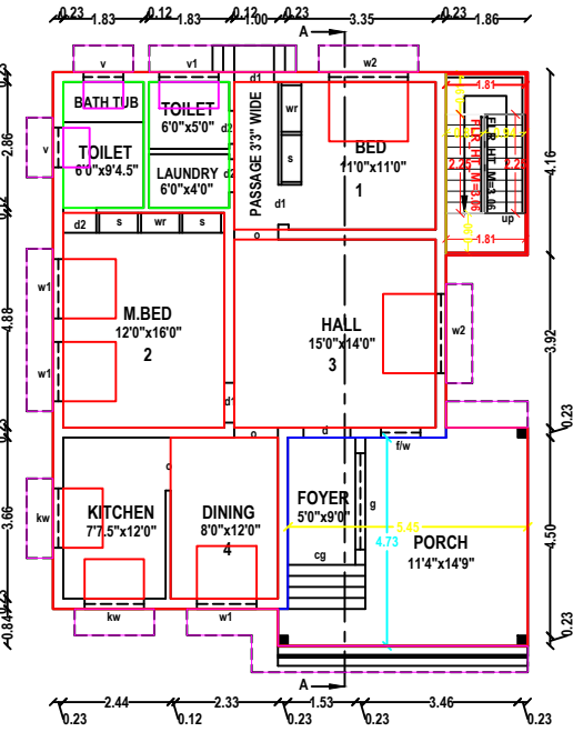
PLAN - GROUND FLOOR RESIDENCE
