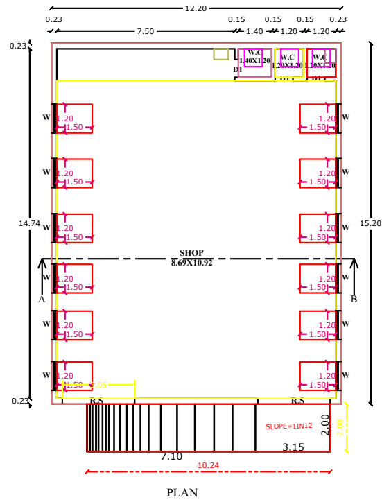
PLAN
