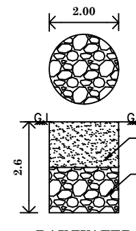
RAINWATER HARVESTING
