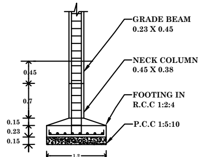
COLUMN DETAILS SCALE-1:30
