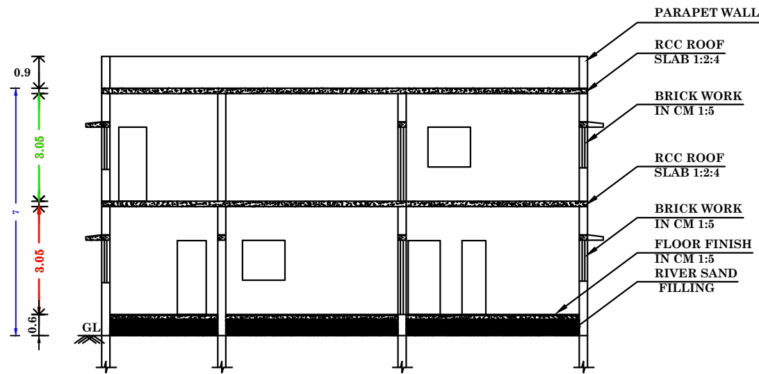
SECTION ON AA1
