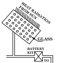
SOLAR SYSTEM
