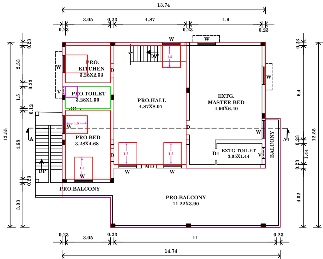
EXISTING AND PROPOSED FIRST FLOOR PLAN
