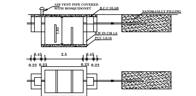
PLAN&SECTION OF SEPTIC TANK TRENCH
