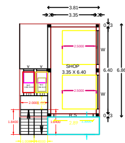
G.FLOOR PLAN
