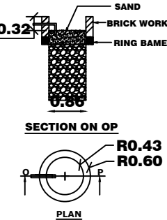
RAIN WATER PIT
