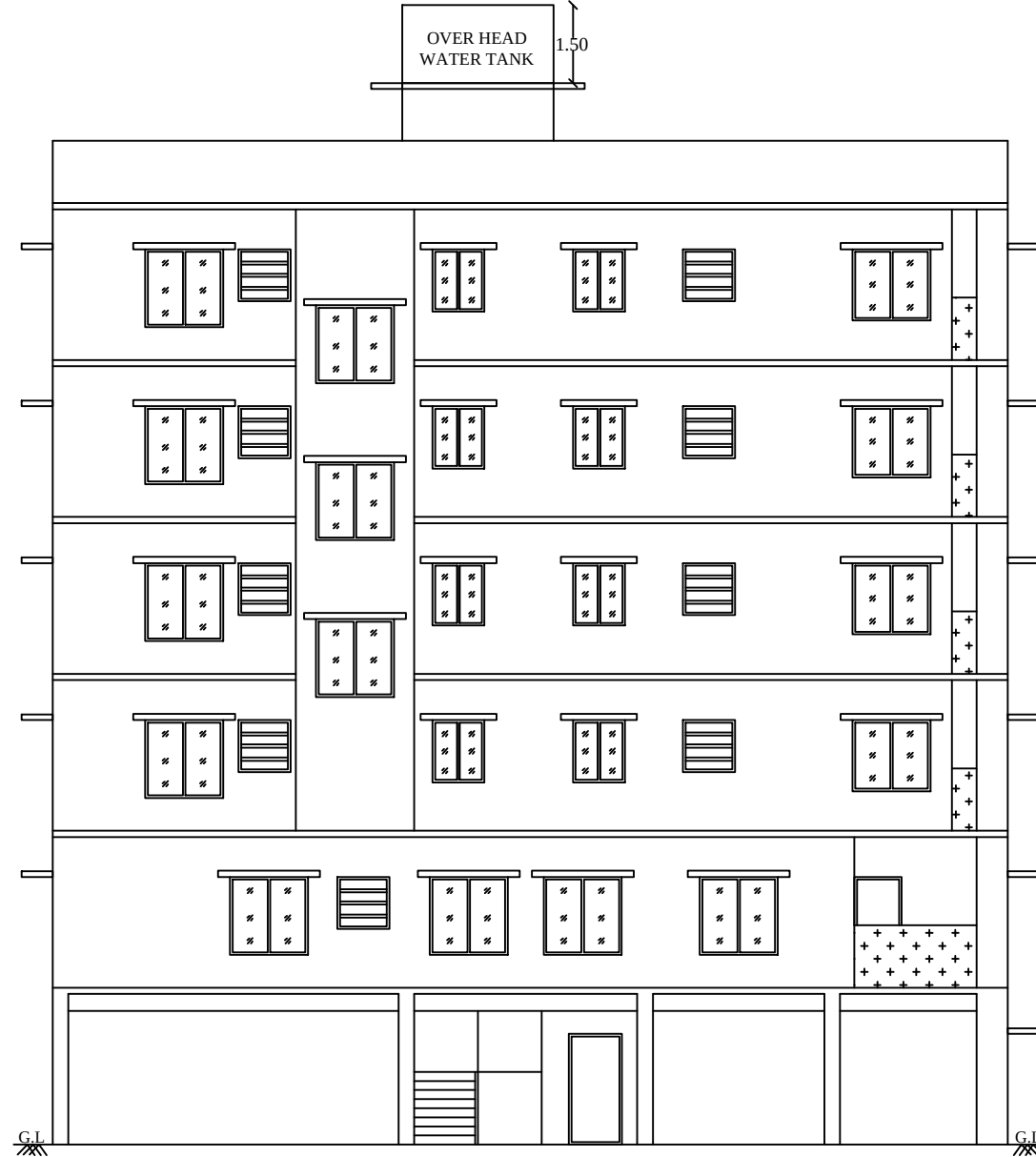
FRONT ELEVATION
