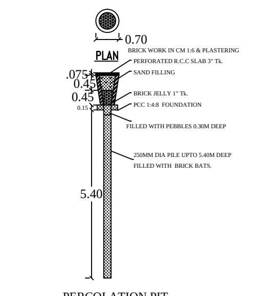
PERCOLATION PIT
