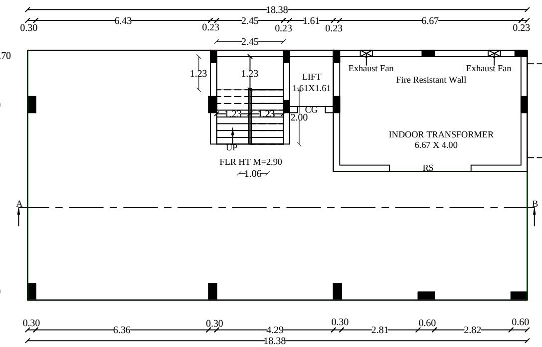
STILT FLOOR PLAN (PARKING)
