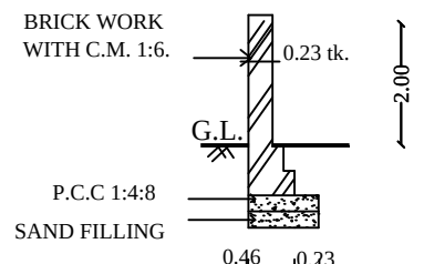
SECTION OF COMPOUND WALL
