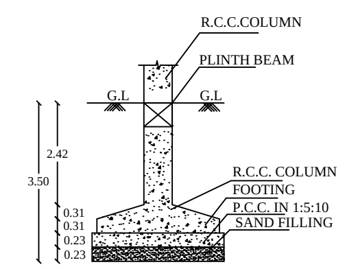
FOUNDATION DETAIL (DETAIL - B)
