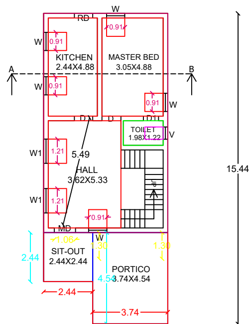
TYPICAL_FLOOR_PLAN=1,2 GROUND FLOOR
