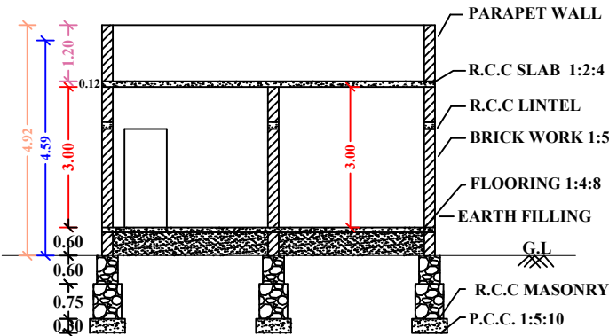
"SECTION "AB"
