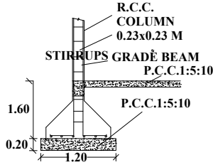
COLUMN DETAIL
