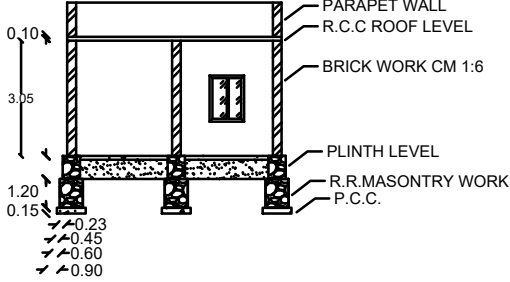
SECTION AB
