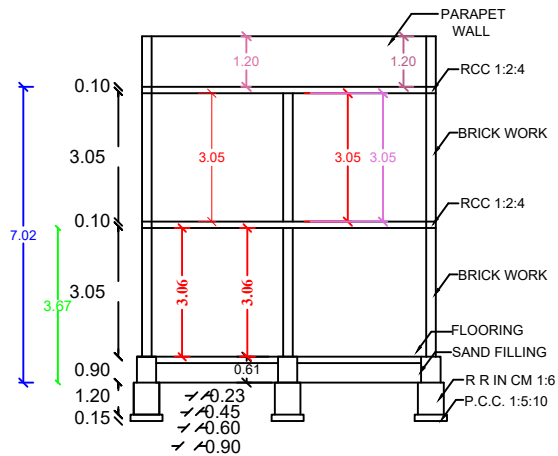
SECTION AB
