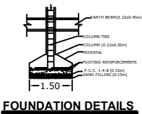
FOUNDATION DETAILS
