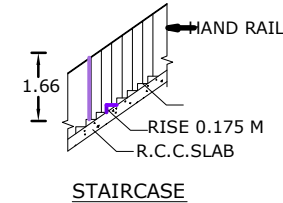
STAIRCASE
