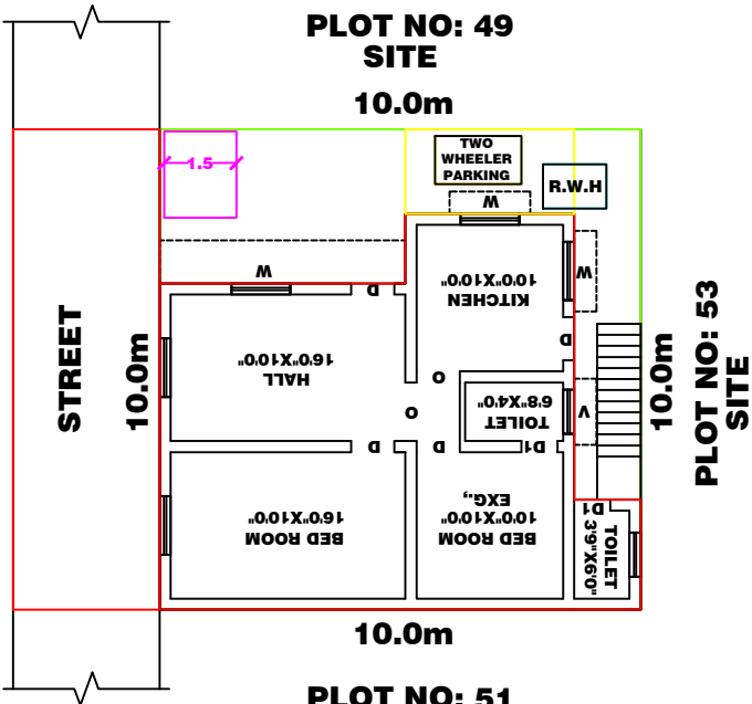
SITE PLAN
