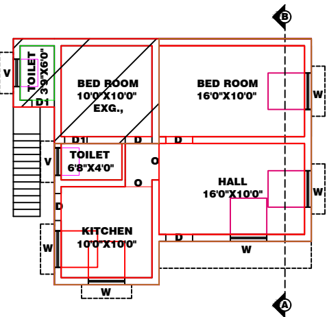
PLAN (EXISTING & PROPOSED)
