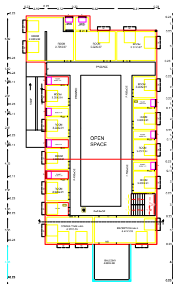
EXT FIRST FLOOR COMMERCIAL PLAN
