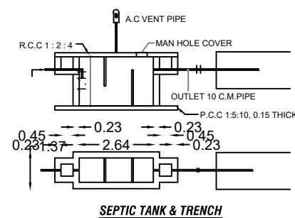
SEPTIC TANK & TRENCH
