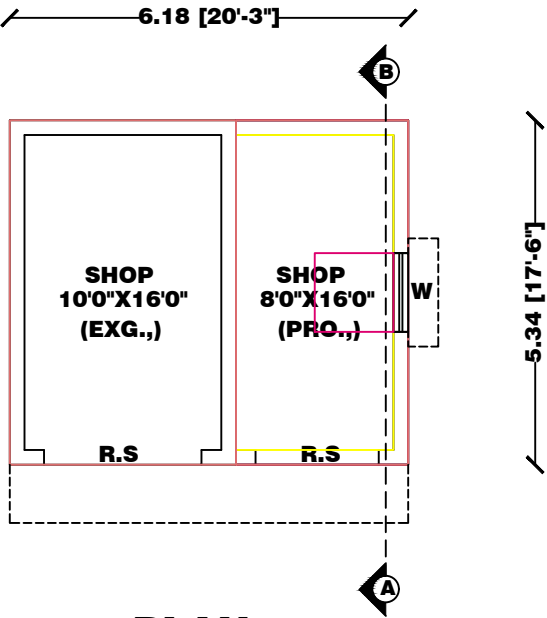
PLAN EXISTING & PROPOSED
