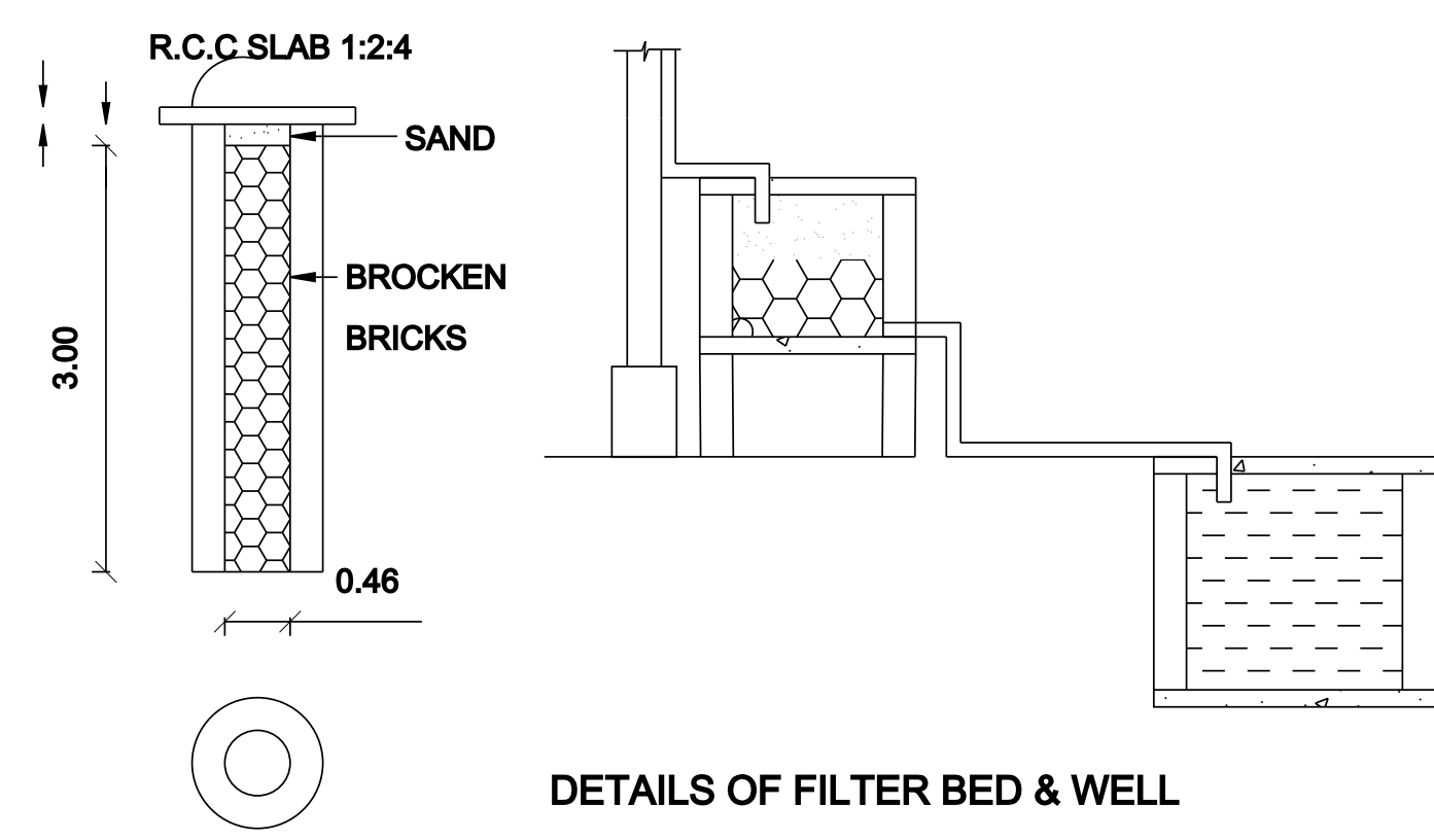
DETAILS OF FILTER BED & WELL
