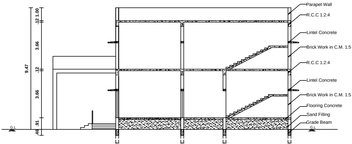
SECTION ON "CD "
