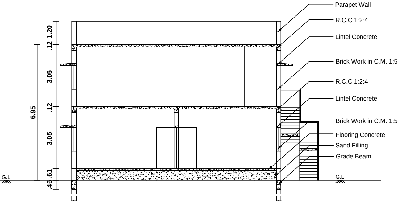
SECTION "AB"
