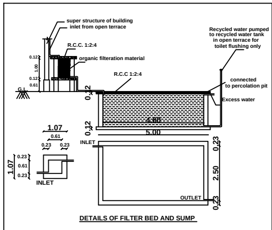
DETAILS OF FILTER BED AND SUMP
