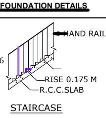
STAIRCASE
