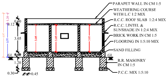
SECTION OF "AB"
