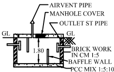
SECTION ON SEPTICTANK
