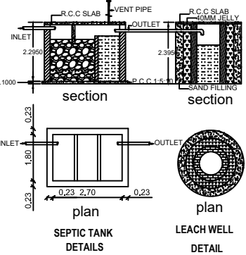
1000 GALLONS CAPACITY SEPTIC TANK (NTS)
